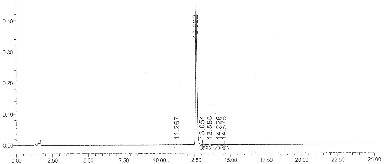
Auto-Scaled Chromatogram
